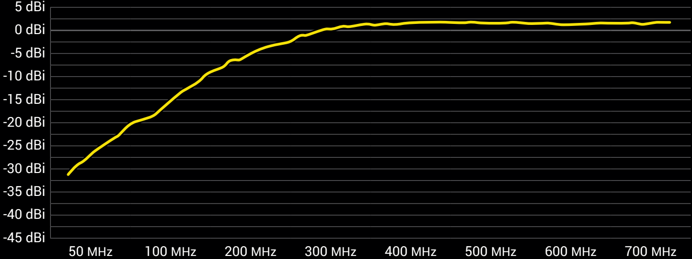
Gain Diagram BicoLOG 5070
