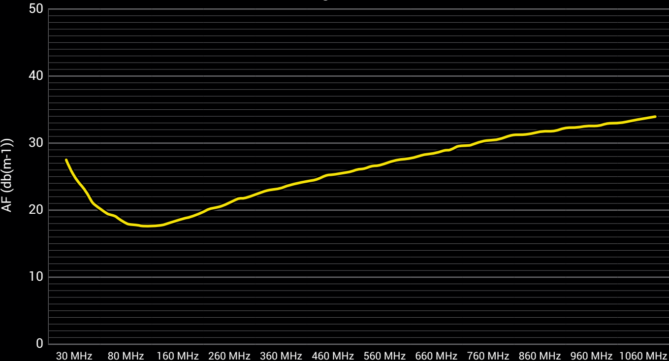
Antenna Factor Diagram BicoLOG 30100 E
